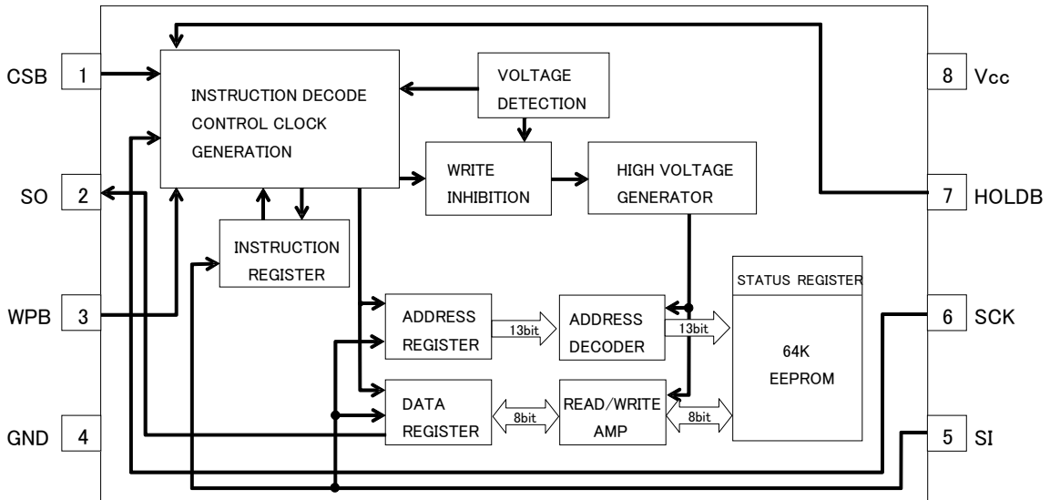
Figure 3. Block Diagram
