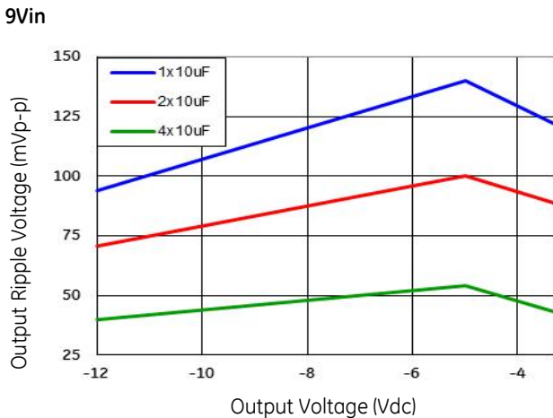
Figure 62. Output ripple with 1x10µF, 2x10µF & 4x10µF output ceramic capacitors (max load).
