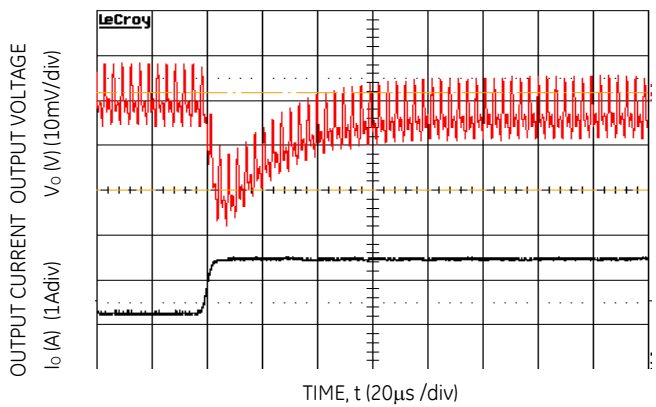
Figure 4. Transient Response to Dynamic Load Change from 50% to 100% at 28Vin, C_{ext} = 10\mu F ceramic + 330µF polymer, C_{Tune}=5600pF & R_{Tune}=261\Omega
