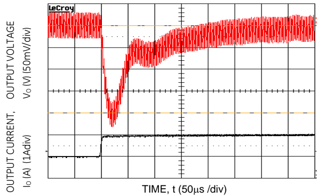
Figure 16. Transient Response to Dynamic Load Change from 50% to 100% at 28Vin, Cext = 3x10uF ceramic, CTune=47pF & RTune=332Ω
