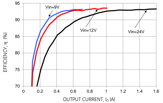
Figure 49. Converter Efficiency versus Output Current.
