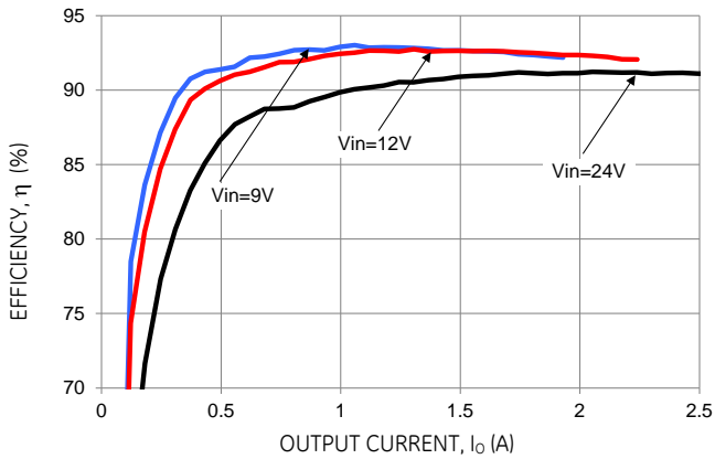
Figure 48. Converter Efficiency versus Output Current.
