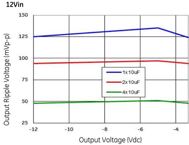
Figure 63. Output ripple with 1x10µF, 2x10µF & 4x10µF output ceramic capacitors (max load).
